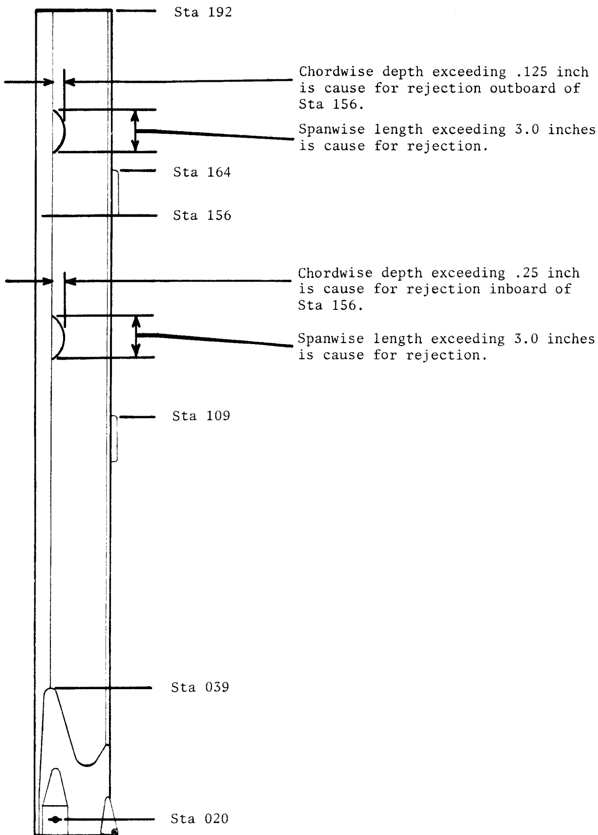
Figure 2. Skin-Spar Bond Separation Criteria
