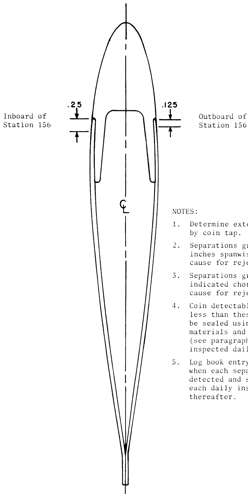
Figure 1. Bond Separation Criteria - Skin to Spar Bond
