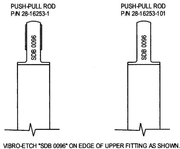
Figure 4. Push-Pull Rod Marking
