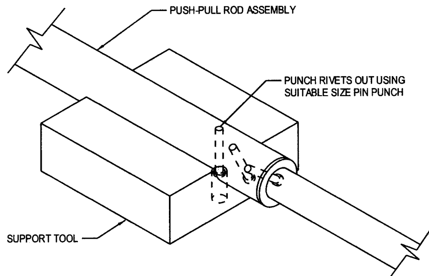
Figure 3. Rivet Removal
