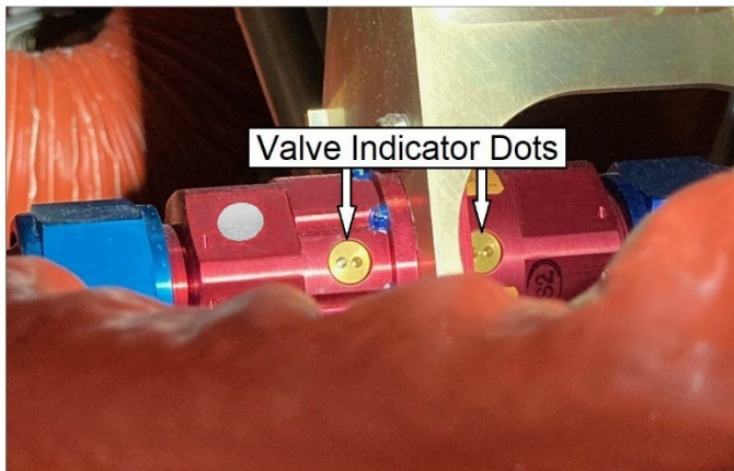
Figure 7-4. Left-Side Fuel Feed Line Coupling Installation
