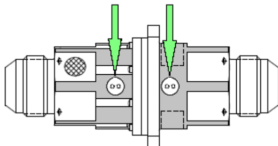
DOTS PARALLEL - VALVES ARE OPEN
