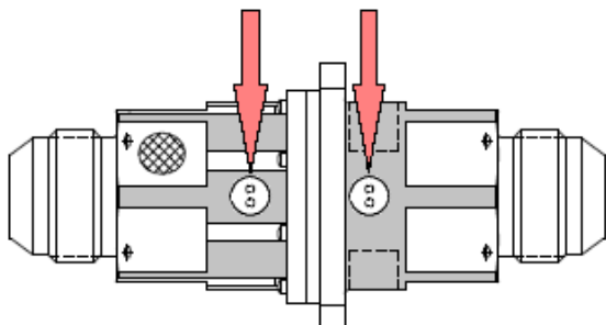
DOTS PERPENDICULAR - VALVES ARE CLOSED
