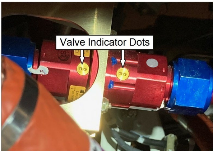
Figure 7-4. Left-Side Fuel Feed Line Coupling Installation
