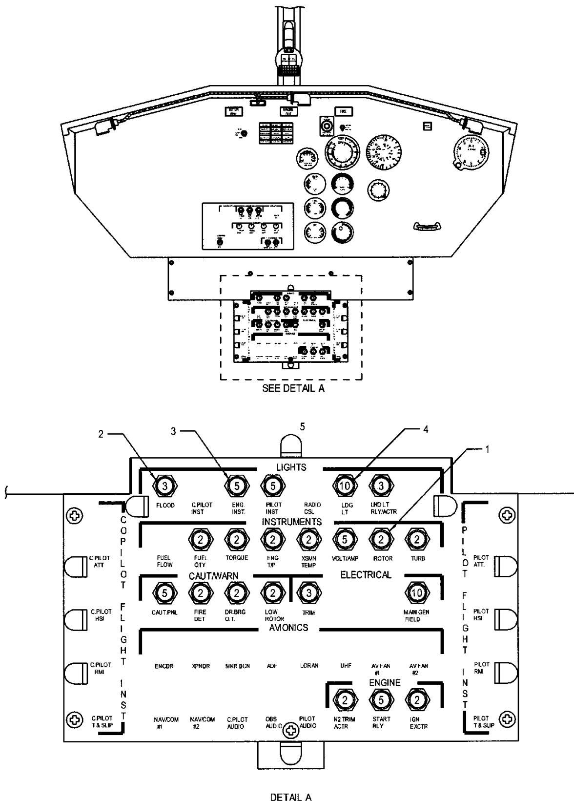
FIGURE 10-5. TH-28 CIRCUIT BREAKER PANEL
