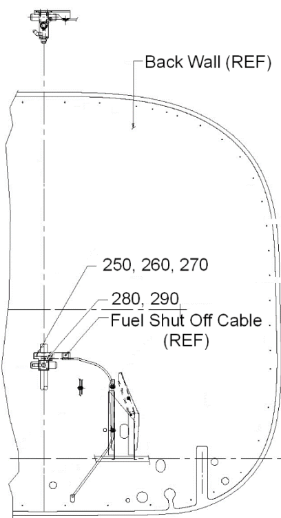
View B-B View Looking Forward
