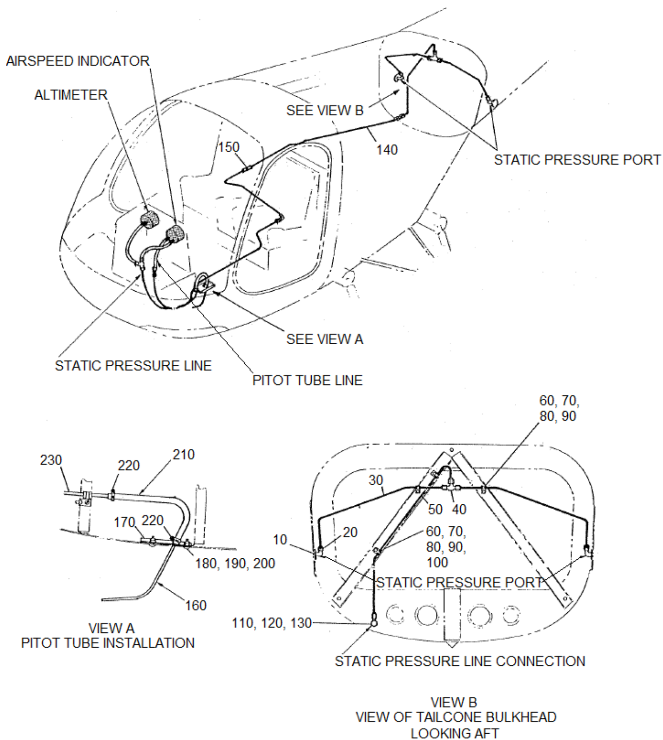
FIGURE 11-11. PITOT STATIC SYSTEM INSTALLATION
