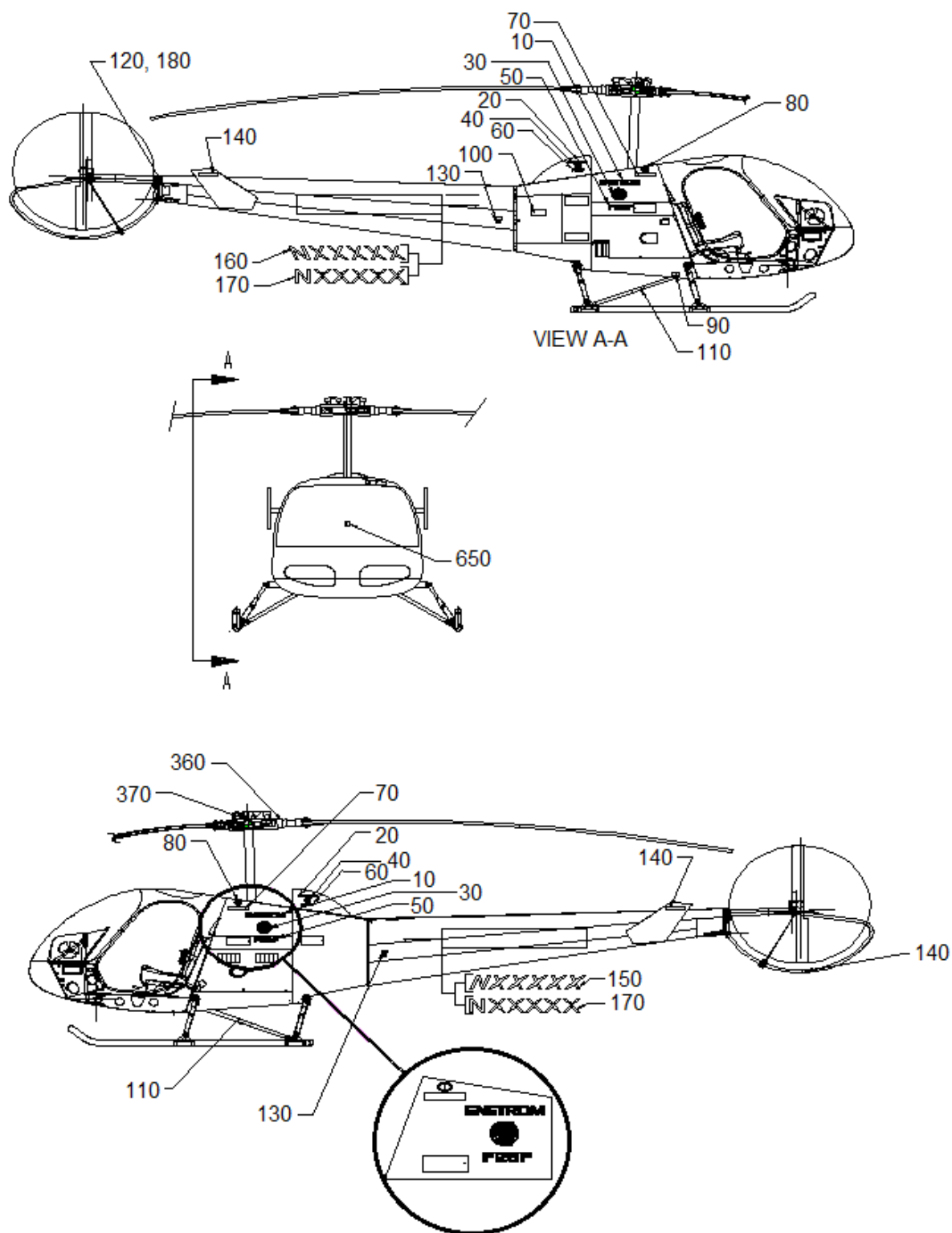
FIGURE 11-21. PLACARD INSTALLATION
