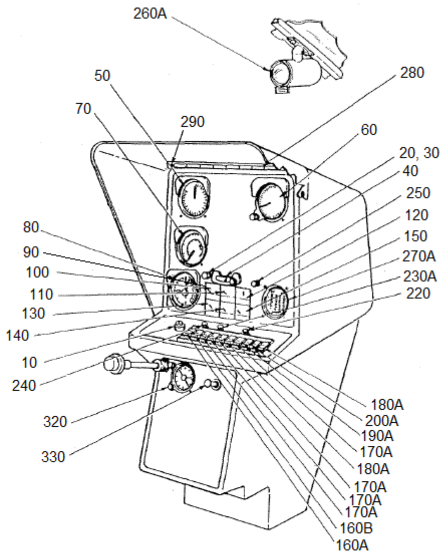
280FX INSTRUMENT PANEL INSTALLATION (12V)
