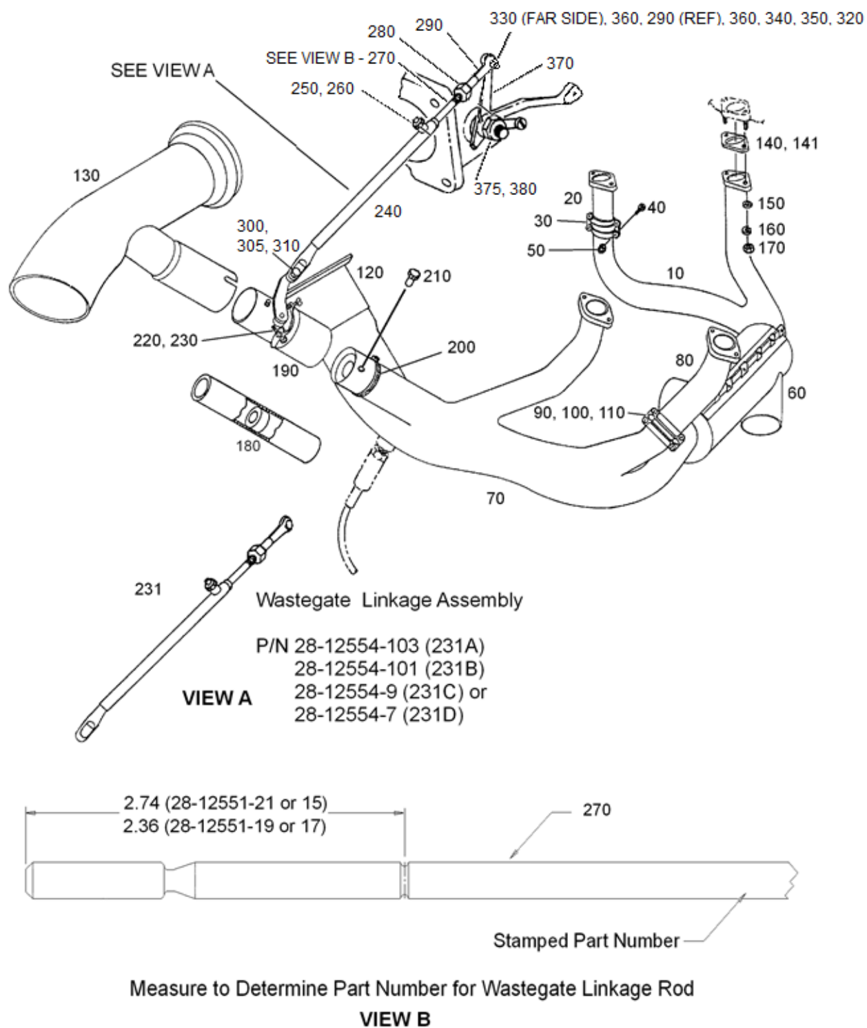
FIGURE 3-28. EXHAUST SYSTEM INSTALLATION (C, F MODELS)
