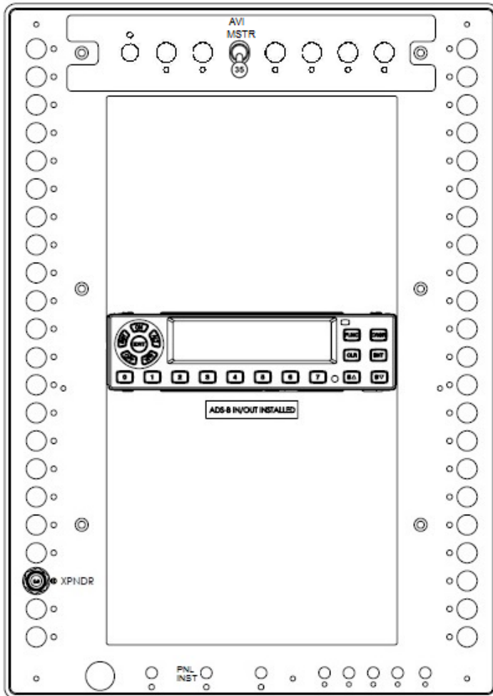
Figure 7-1. GTX 345 Installation
